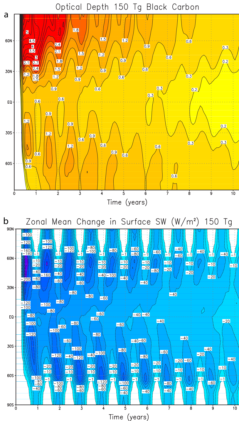
Figure 1. Changes in visible optical depth and net downward shortwave radiation at the surface for the 150 Tg case. Although the maximum forcing is in the Northern Hemisphere during the first summer, the aerosols rapidly spread around the globe producing large solar radiation reductions in both hemispheres.
