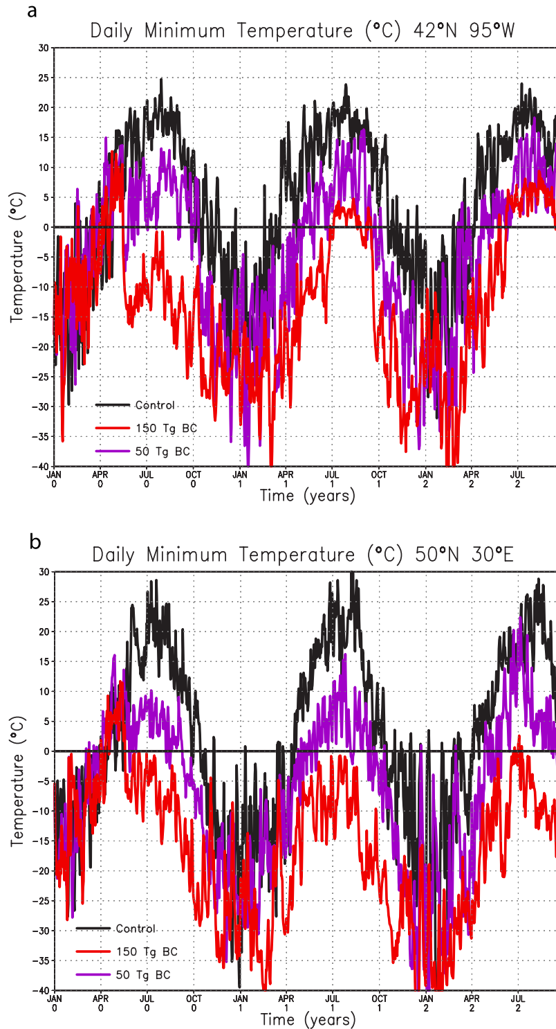
Figure 5. Time series of daily minimum temperature from the control, 50 Tg, and 150 Tg cases for two important agricultural regions, (top) Iowa, United States, at 42°N, 95°W, and (bottom) Ukraine at 50°N, 30°E. These two locations are shown on the map in Figure 4.
