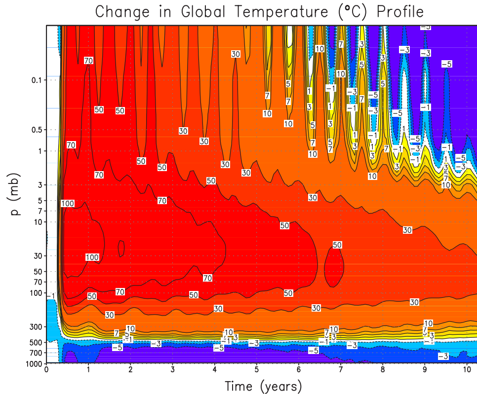
Figure 3. Change in global average temperature (°C) profile for the 150 Tg case from the surface to 0.02 mbar [80 km]. The semiannual periodicity at the top is due to enhanced heating during the summers in each hemisphere.
