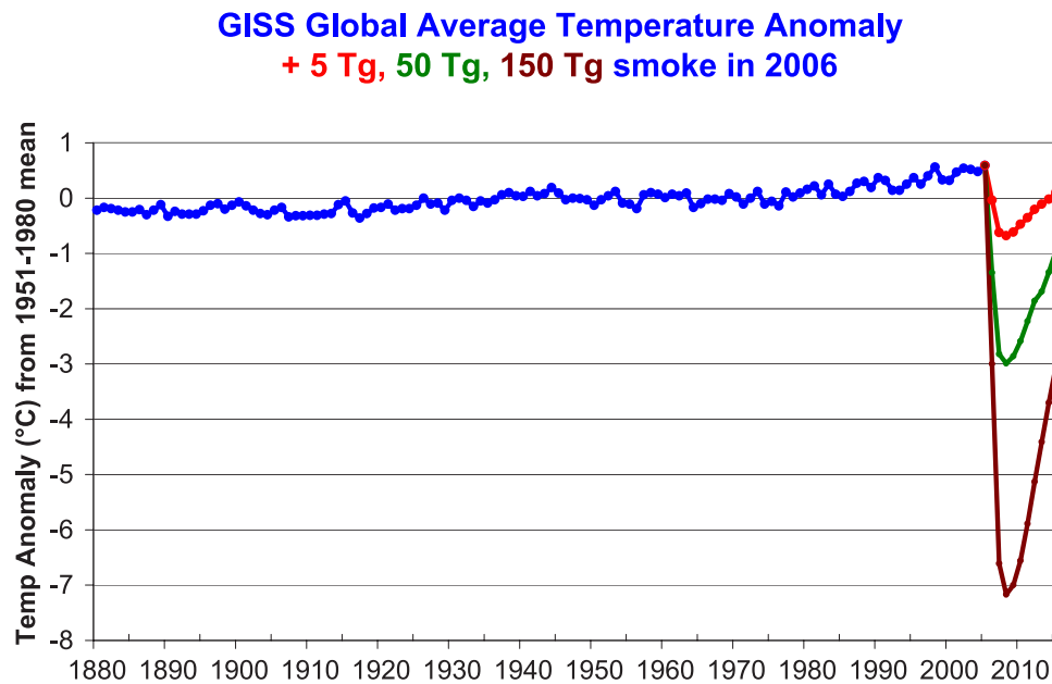
Figure 8. Global average surface air temperature change from the 5 Tg (red), 50 Tg (green), and 150 Tg (brown) cases in the context of the climate change of the past 125 years. Observations are from the National Aeronautics and Space Administration Goddard Institute for Space Studies analysis [Hansen et al. , 2001, updated at http://data.giss.nasa.gov/gistemp/2005/ ].
