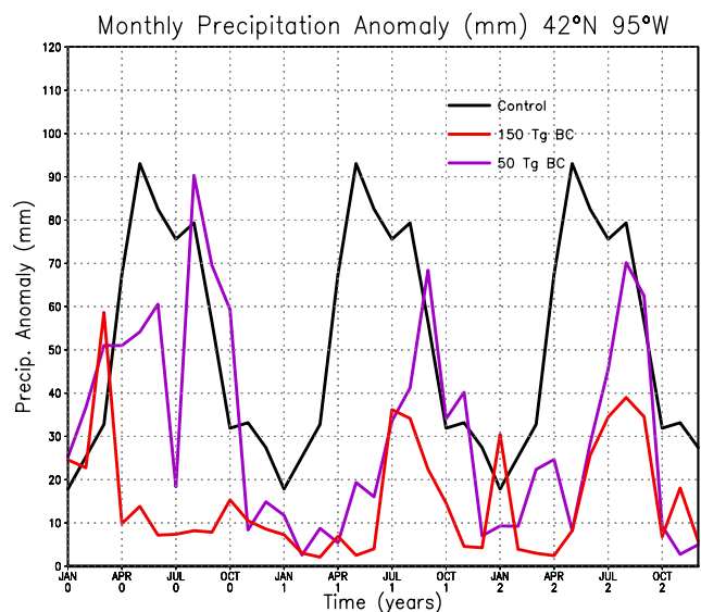
Figure 7. Time series of monthly precipitation from the control, 50 Tg, and 150 Tg cases for the important agricultural region of Iowa, United States, at 42°N, 95°W. The location is shown on the map in Figure 6.
