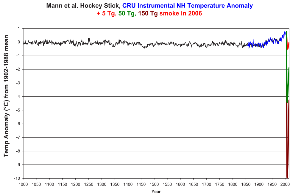
Figure 9. Northern Hemisphere average surface air temperature change from 5 Tg (red), 50 Tg (green), and 150 Tg (brown) cases in the context of the climate change of the past 1000 years. The “hockey stick” nature of the curve is barely discernible when plotted on this scale. Black curve is from Mann et al. [1999], and the blue curve is from the latest data from the Climatic Research Unit website ( http://www.cru.uea.ac.uk/cru/data/temperature/ ).
