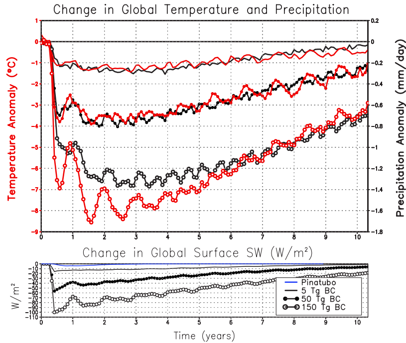
Figure 2. Change of global average surface air temperature, precipitation, and net downward shortwave radiation for the 5 Tg [Robock et al. , 2007], 50 Tg and 150 Tg cases. Also shown for comparison is the global average change in downward shortwave radiation for the 1991 Mt. Pinatubo volcanic eruption [Oman et al. , 2005], the largest volcanic eruption of the 20th century. The global average precipitation in the control case is 3.0 mm/day, so the changes in years 2–4 for the 150 Tg case represent a 45% global average reduction in precipitation.
